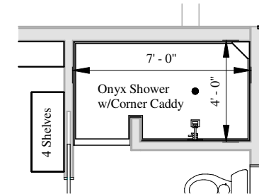
② Optional Onyx Shower 3/16" = 1'-0"
