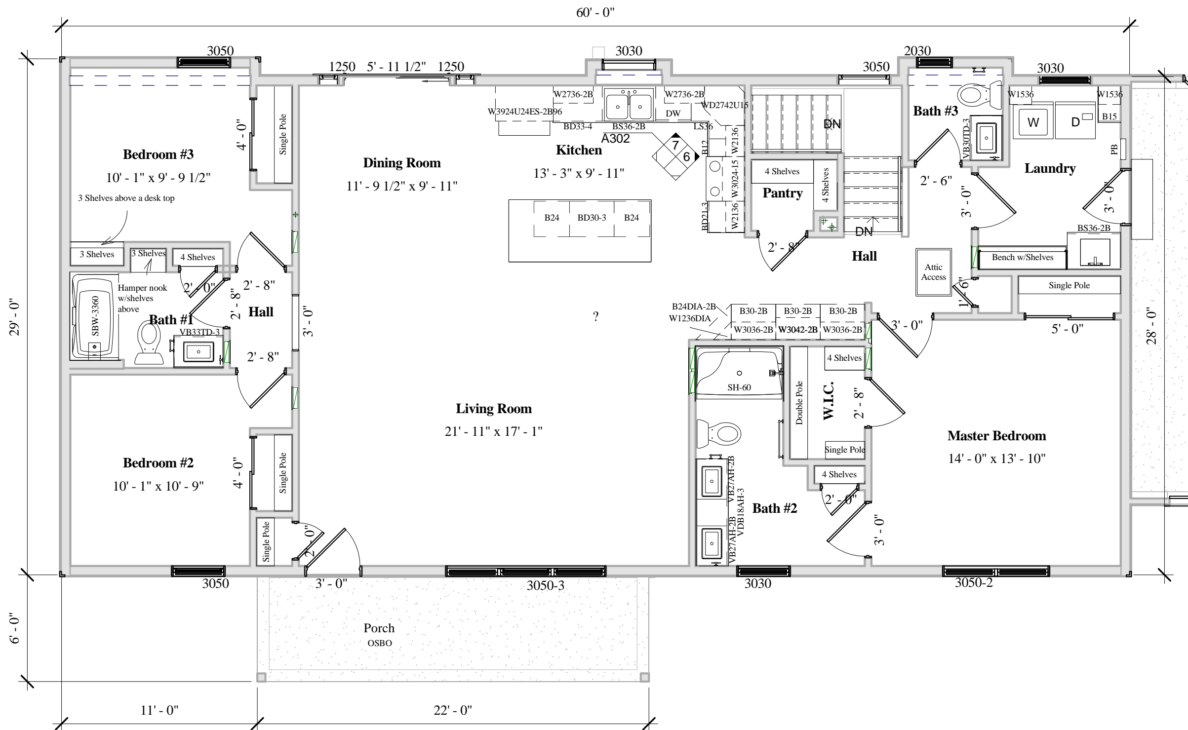
① 5713 Floor Plan 3/16" = 1'-0"
